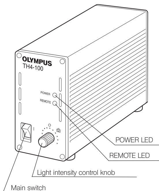
Halogen Lamp Power Supply Unit TH4
