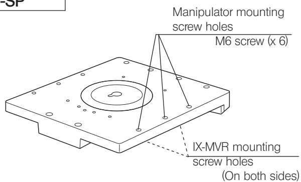
Plain Stage IX2-SP
